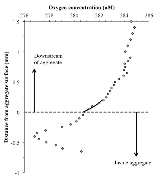
Figure 5. Example oxygen profile (µM) through a phytodetrital aggregate collected at 46 m depth. Measurements were made with microsensors in steps of 50–100 µm, with negative values reflecting the distance into the aggregate from the surface. The solid black line shows the model fit used to calculate the oxygen flux in the diffusive boundary layer.
